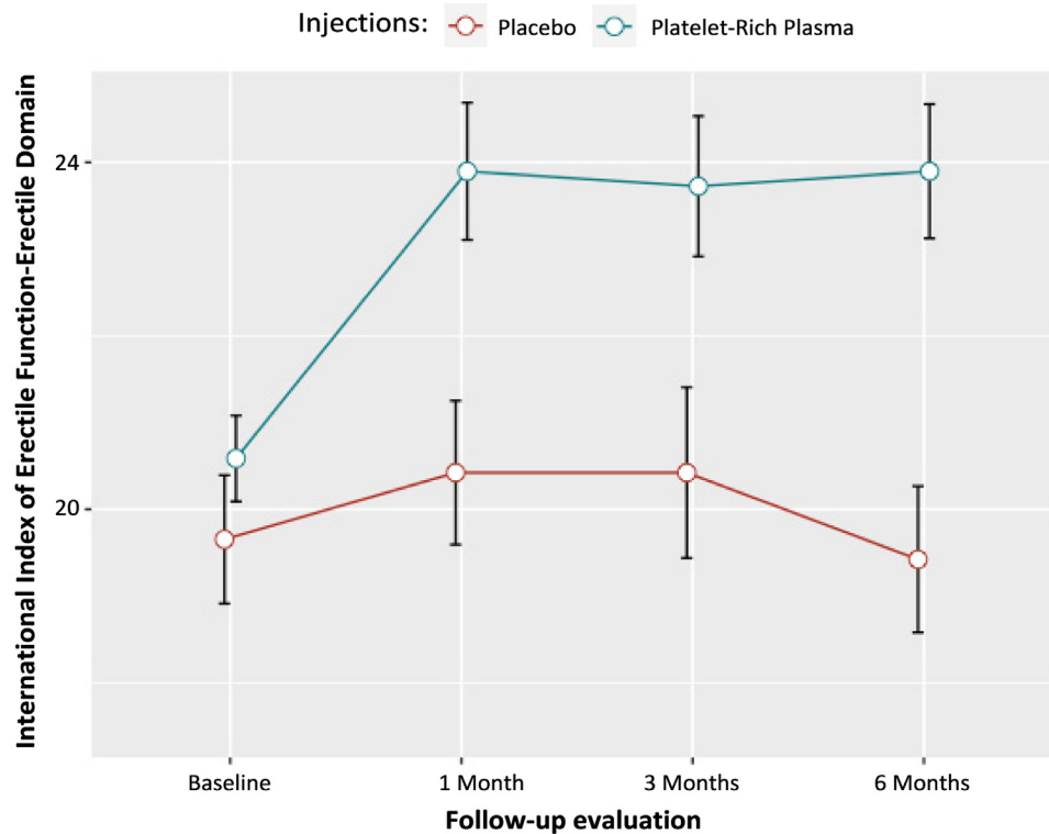
Figure 3. The effect of PRP versus placebo on IIEF-EF. PRP = Platelet-Rich Plasma; IIEF-EF = International Index of Erectile Function-Erectile Domain. [Figure 3 is available in color online at www.jsm.jsexmed.org .]
